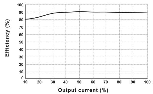
Efficiency vs Output Load (Vin=12V, DB1-12D05XT)
