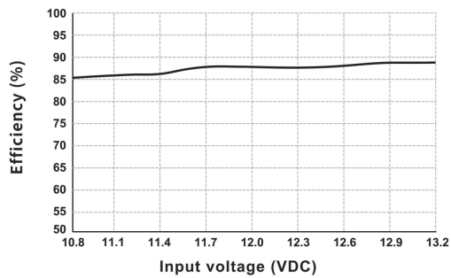
Efficiency vs Input Voltage (Full Load, DB1-12D05XT)
