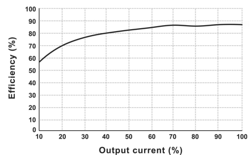
Efficiency VS Output Load (Vin=24V,DB1-24S12XT)
