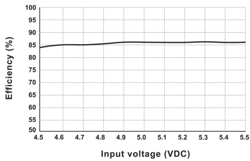
Efficiency VS Input Voltage (Full Load, DB2-05D05LS)
