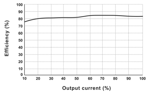
Efficiency VS Output Load (Vin=5V, DB2-05D05LS)
