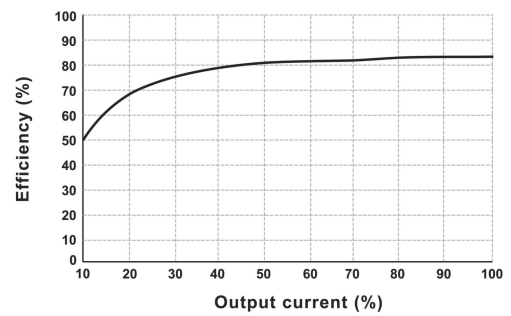
Efficiency VS Output Load (Vin=5V, DB2-05S05S)
