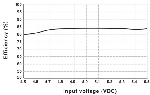
Efficiency VS Input Voltage (Full Load, DB2-05S05S)
