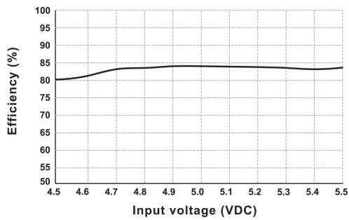
Efficiency vs Input Voltage (Full Load, DB2-05S05XT)
