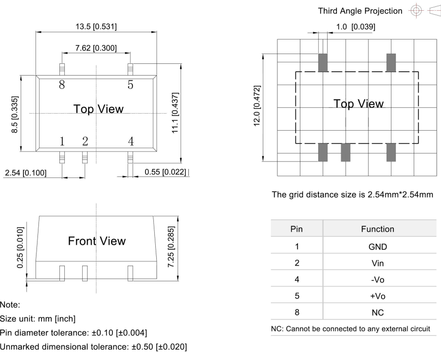
DB2-xxSxxXT Dimensions and Recommended Layout
