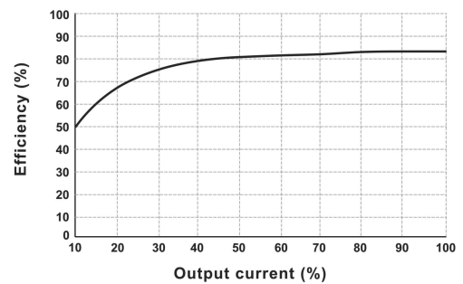
Efficiency vs Output Load (Vin=5V, DB2-05S05XT)
