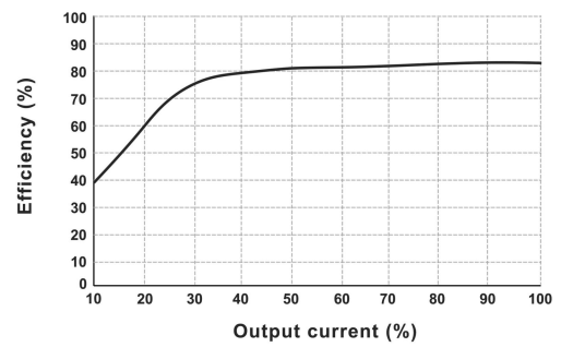
Efficiency VS Output Load (Vin=5V,DF1-05D05LS)
