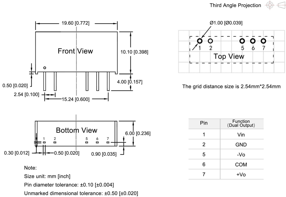
DF1-xxDxxLS Dimensions and Recommended Layout
