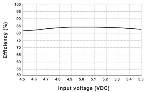
Efficiency VS Input Voltage (Full Load, DF1-05D05LS)
