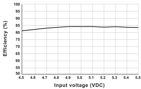
Efficiency vs Input Voltage (Full Load, DF1-05D05XT)
