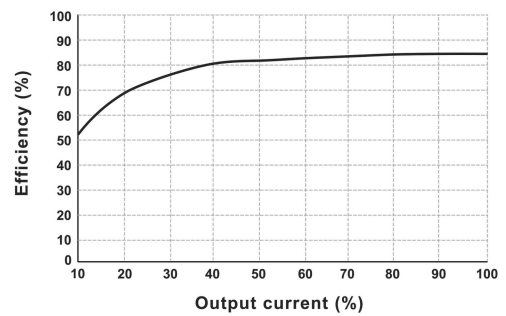
Efficiency vs Output Load (Vin=12V, DF1-05D05XT)
