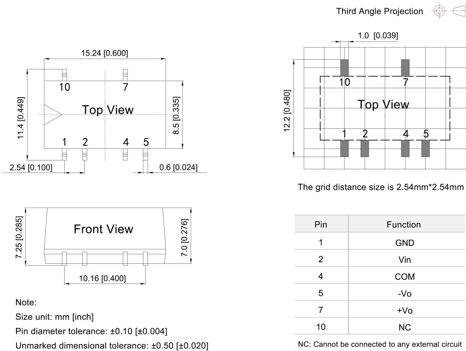
DF1-xxDxxXT Dimensions and Recommended Layout
