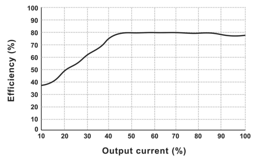
Efficiency VS Output Load (Vin=5V, DF1-05S05D)
