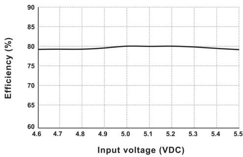
Efficiency VS Input Voltage (Full Load, DF1-05S05D)
