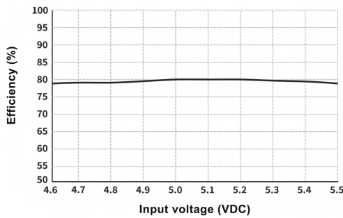
Efficiency VS Input Voltage (Full load, DF1-05S05S)
