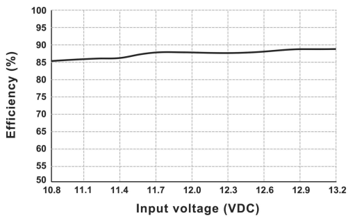
Efficiency vs Input Voltage (Full Load, DF1-12S05XT)
