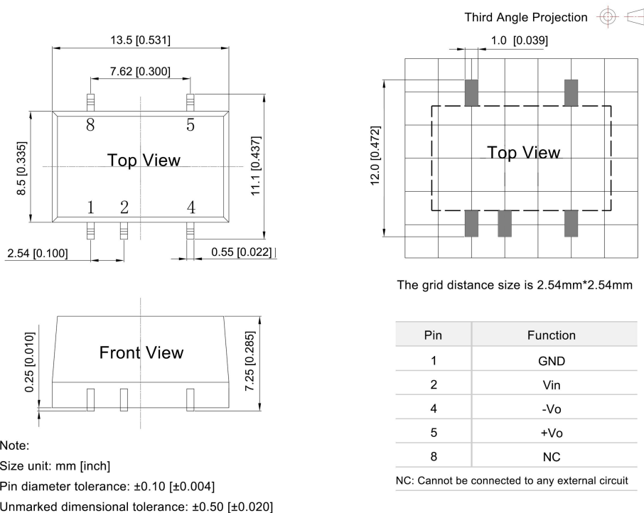
DF1-xxSxxXT Dimensions and Recommended Layout
