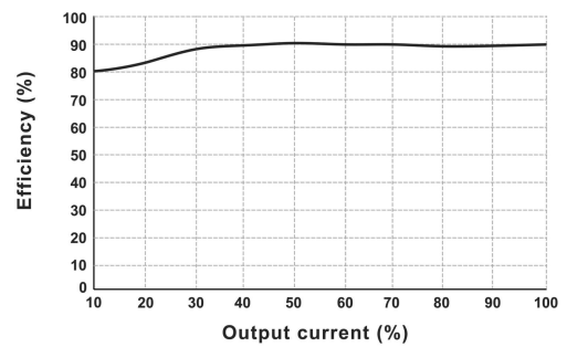
Efficiency vs Output Load (Vin=12V, DF1-12S05XT)
