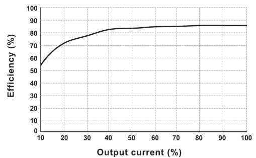
Efficiency vs Output Load (Vin=5V, DF2-05D05LT)
