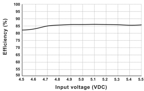
Efficiency vs Input Voltage (Full Load, DF2-05D05LT)
