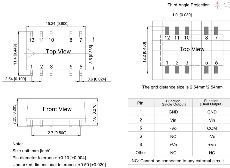
DF2-xxDxxLT Dimensions and Recommended Layout
