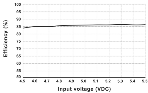
Efficiency vs Input Voltage (Full Load, DF2-05D05XT)
