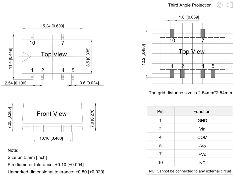
DF2-xxDxxXT Dimensions and Recommended Layout
