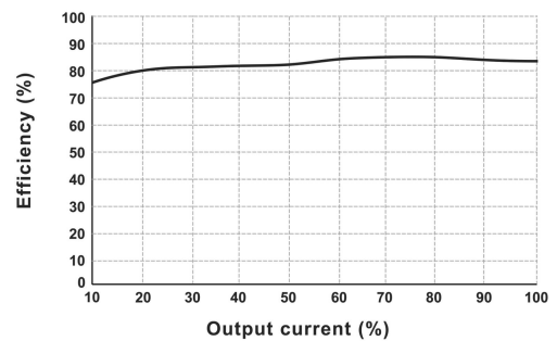
Efficiency vs Output Load (Vin=12V, DF2-05D05XT)
