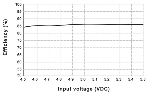
Efficiency VS Input Voltage (Full Load, DF2-05S05D)
