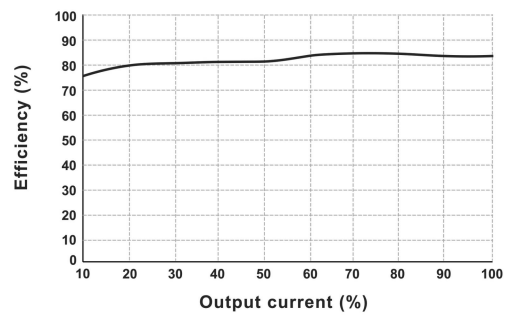
Efficiency VS Output Load (Vin=5V, DF2-05S05D)
