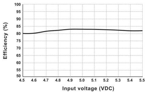
Efficiency vs. Input Voltage (Full Load, DF2-05S05S)
