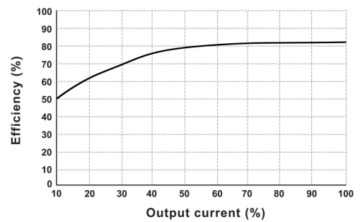
Efficiency vs. Output Load (DF2-05S05S)
