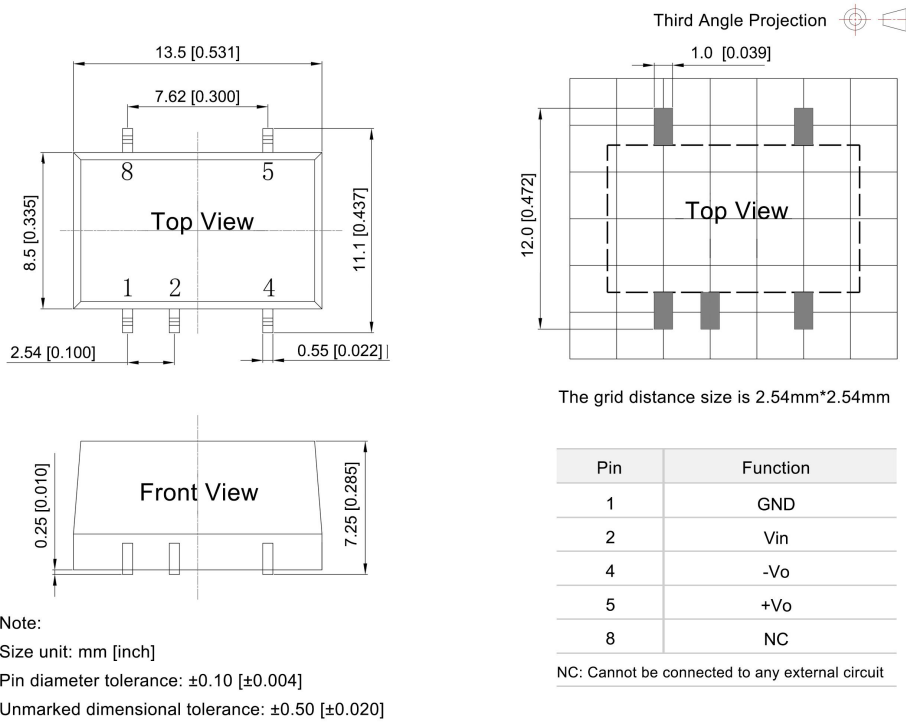
DF2-xxSxxXT Dimensions and Recommended Layout
