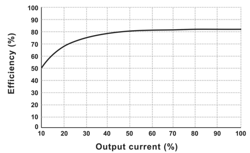
Efficiency vs Output Load (Vin=5V, DF2-05S05XT)
