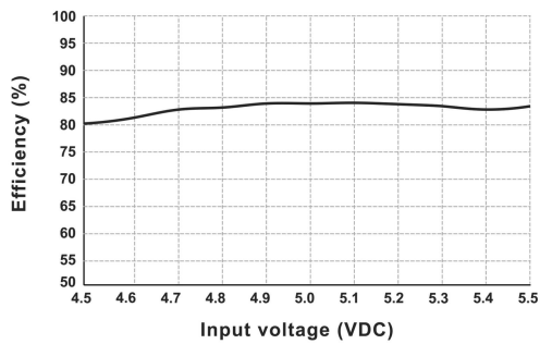
Efficiency vs Input Voltage (Full Load, DF2-05S05XT)
