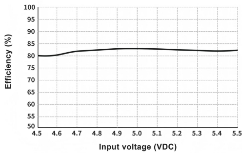
Efficiency vs. Input Voltage (Full Load, DFR2-05S05S)
