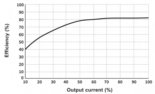
Efficiency vs. Output Load (Vin=5V,DFR2-05S05S)
