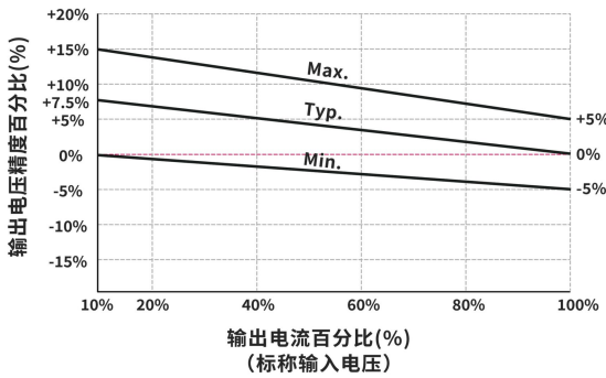
误差包络曲线图 (DH1-05D09LS/DH1-05D12LS)
