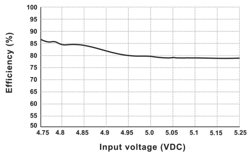
Efficiency VS Input Voltage (Full load, DRF1-05S05LS)
