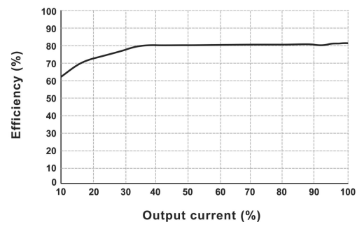
Efficiency VS Output Load (Vin=5V, DRF1-05S05LS)
