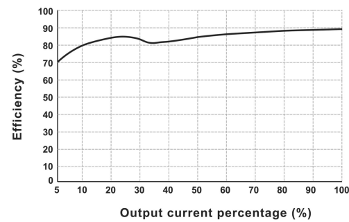
Efficiency VS Output Load (Vin=24V, VB10-24S05S)
