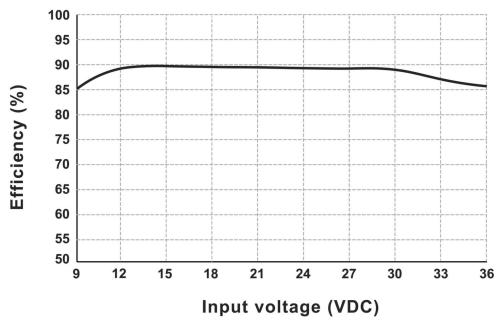
Efficiency VS Input Voltage (Full load, VB10-24S05S)
