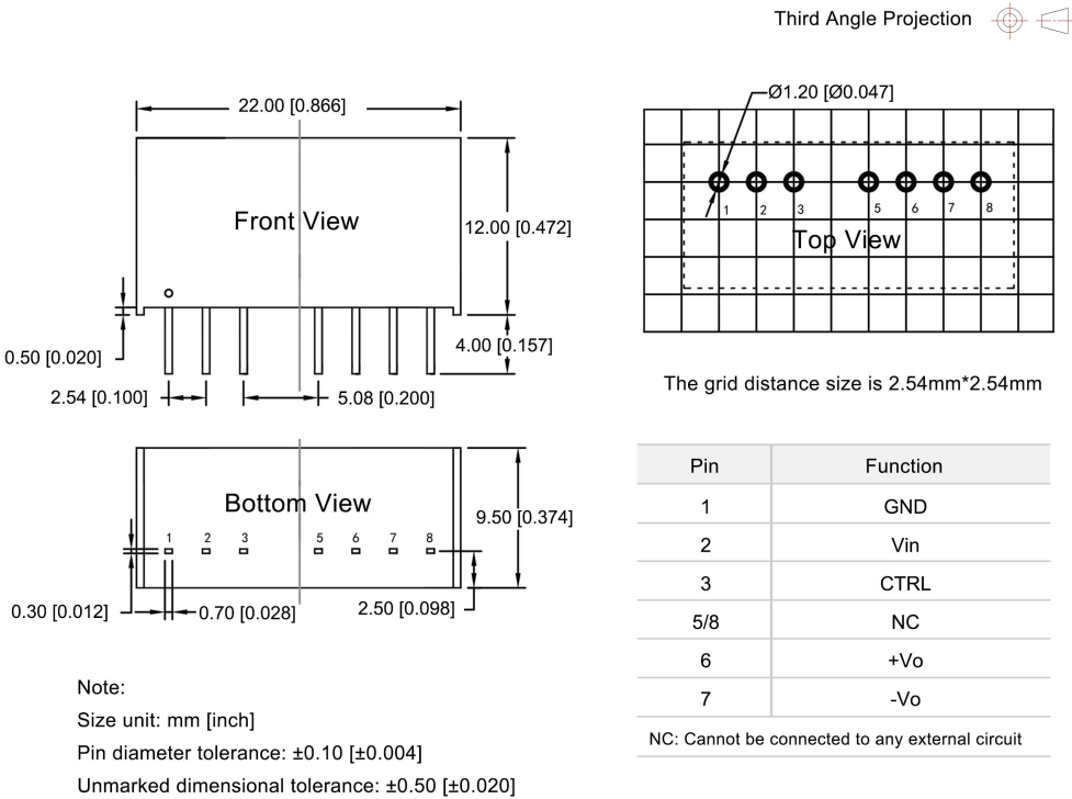
VB10-xxSxxS Dimensions and Recommended Layout
