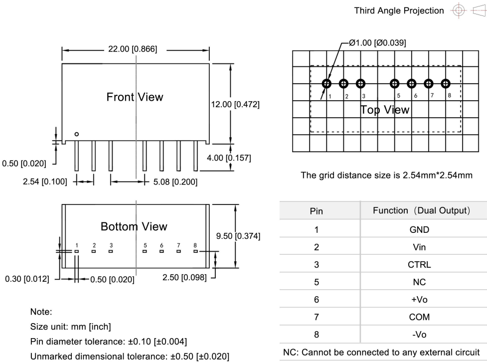
VB3-xxDxxS Dimensions and Recommended Layout
