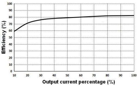
Efficiency vs. Output Load (Vin=12V, VB3-24D05S)
