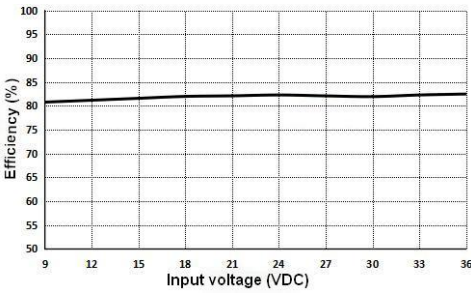
Efficiency vs. Input Voltage (Full Load, VB3-24D05S)
