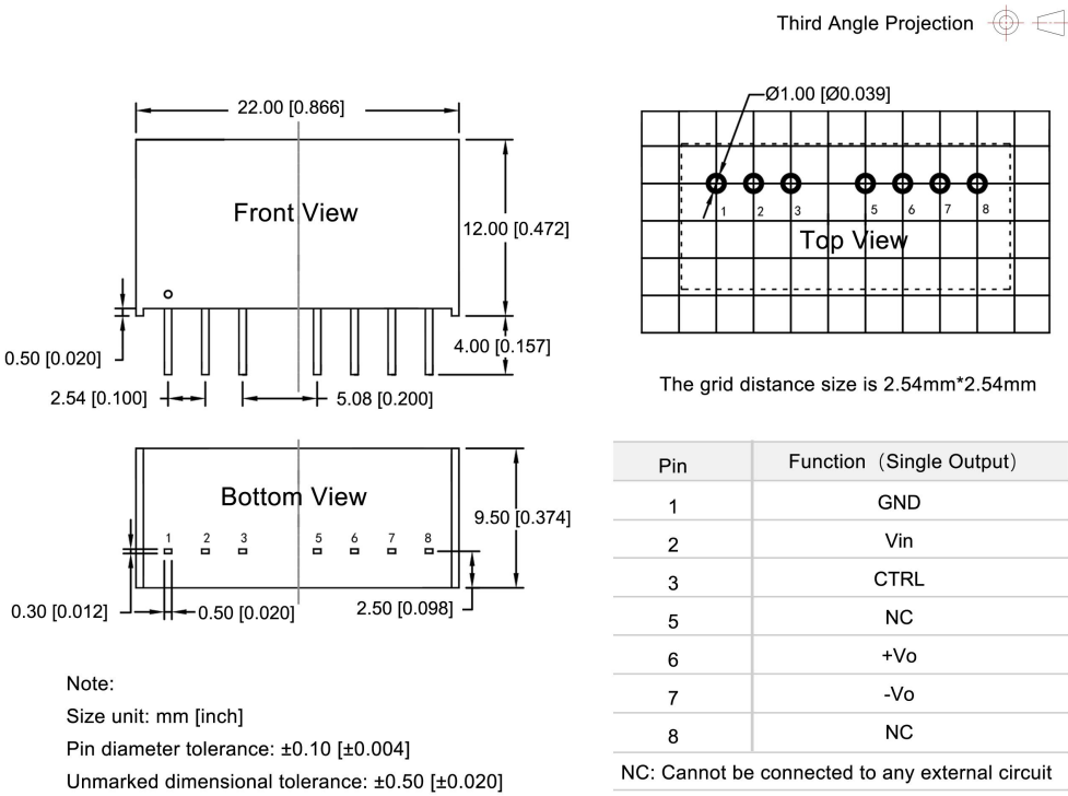
VB3-xxSxxS Dimensions and Recommended Layout
