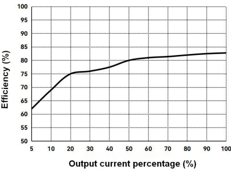
Efficiency VS Output Load (Vin=48V, VB3-48S24S)
