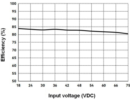
Efficiency VS Input Voltage (Full Load, VB3-48S24S)
