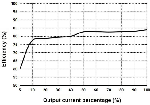
Efficiency VS Output Load (Vin=48V, VB3-48S24S)
