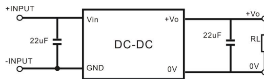
Application circuit 1
