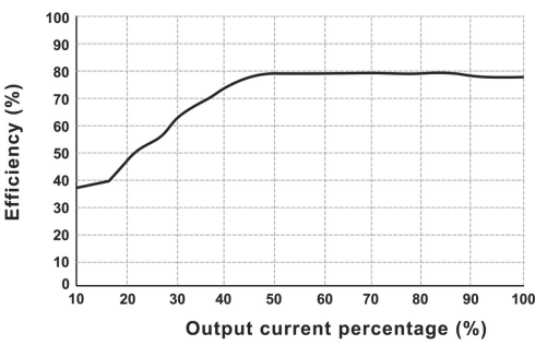
Efficiency VS Output Load Curve (Vin=24V, VB6-24S05S)
