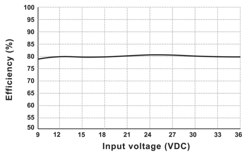
Efficiency VS Input Voltage Curve (Full Load, VB6-24S05S)
