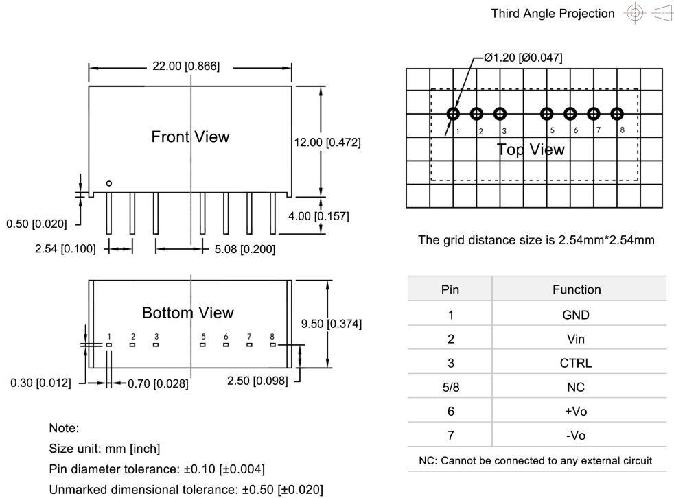
VB6-xxSxxS Dimensions and Recommended Layout
