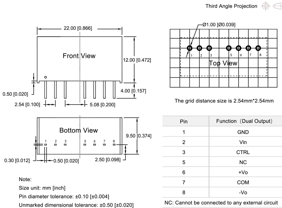
VF1-xxDxxS Dimensions and Recommended Layout
