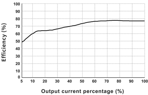
Efficiency VS Output Load (Vin=24V, VF1-24D05S)
