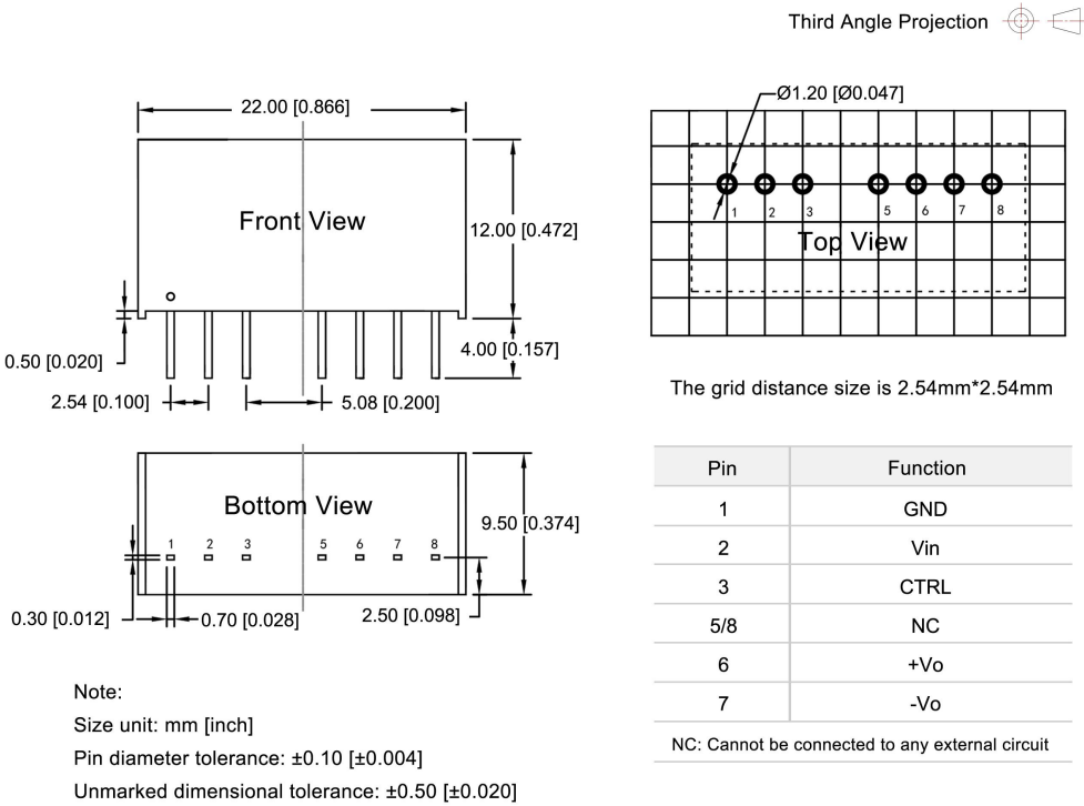
WF3-xxSxxS Dimensions and Recommended Layout
