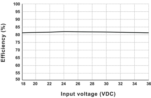
Efficiency VS Input Voltage Curve (Full Load, WF3-24S05S) Efficiency VS Output Load Curve (Vin=24V, WF3-24S05S)
