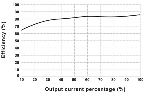
Efficiency vs. Output Load Curve (Vin=24V, WF6-24D15S)
