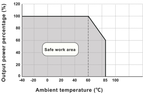
Temperature Derating Curve (24V Nominal Input)
